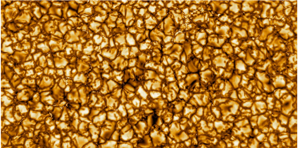
First light: 29/01/2020. Details tot 30 km. Credit: NSO/AURA/NSF.
